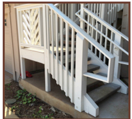
90° landing, showing the notchout that is typically needed for the post.
